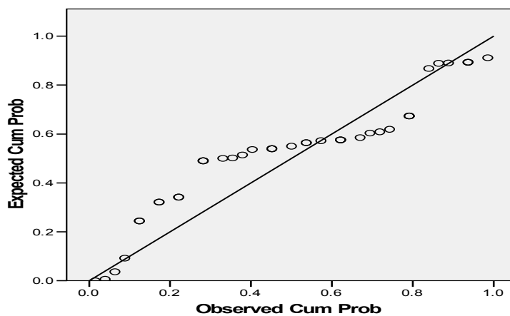
Normal P- P Plot of sediment
