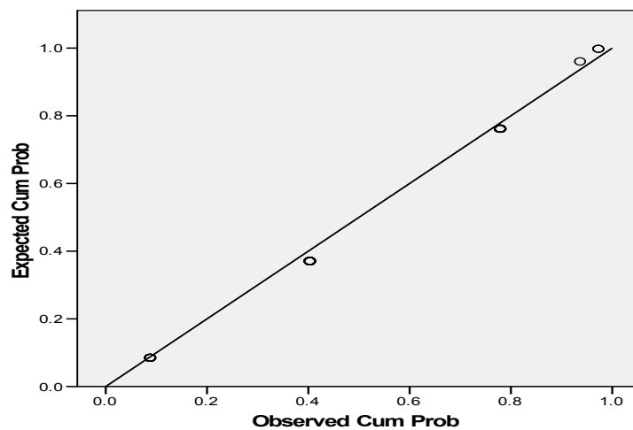
Normal P- P Plot of slopgeo
