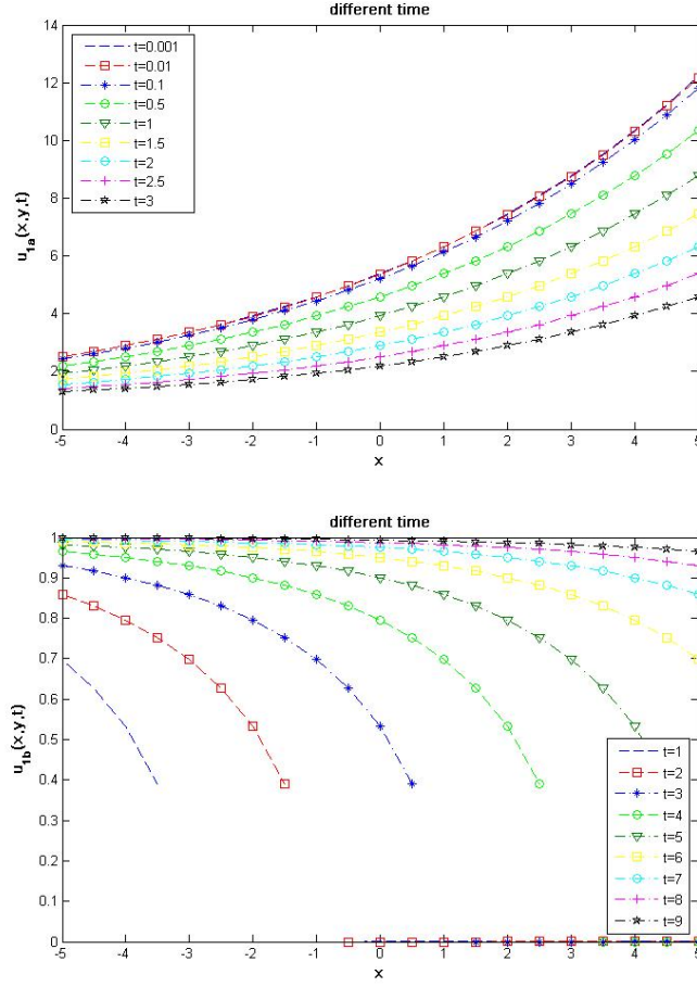
FIGURE 3. The evolution from t = 0.001 to t = 3 when a = 2 and y = 10 for u_{1a} and t = 1 to t = 9 when a = 2 and y = 5 for u_{1b} Eqs. (4.18) and (4.19).
