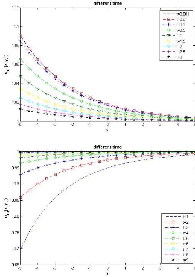
FIGURE 4. The evolution from t = 0.001 to t = 3 when a = 2 and y = 10 for u_{1c} and t = 1 to t = 9 when a = 2 and y = 5 for u_{1d} Eqs. (4.20) and (4.21).
