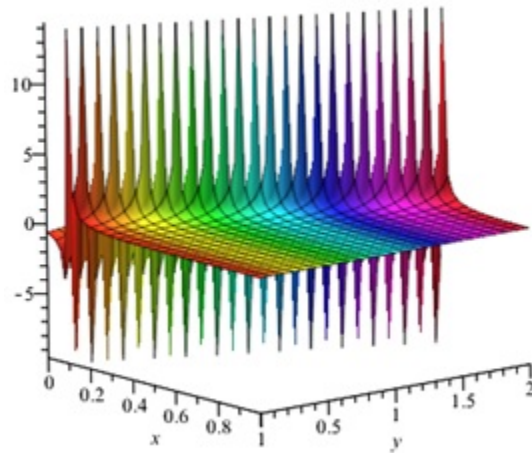
FIGURE 4. propagating wave u_6 at B = 1, C = 1, D = 1, \psi = 1, \lambda = 1, z = 0.1, t = .2, a_0 = 6, b_2 = -6 , and A = -0.25 .
