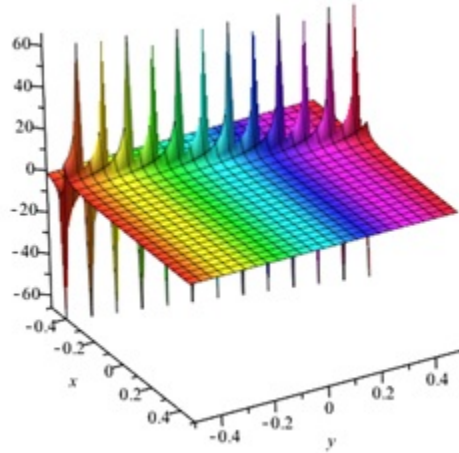
FIGURE 1. Propagating wave u_2 at A = -\frac{1}{4} , B = 1 , C = 1 , D = 1 , \psi = 1 , \lambda = 1 , a_0 = 1 , a_1 = 0 , b_1 = 6 , z = 0.1 , and t = 0.2 .
