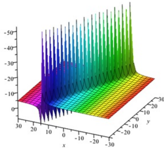
FIGURE 8. Soliton wave solution u_{13} for A = 0.5 , B = 1 , C = 1 , D = 1 , \psi = 1 , \lambda = 2 , a_0 = 1 , a_1 = 6 , z = 1 , t = 2 , c_1 = 1 , and c_2 = 2 .
