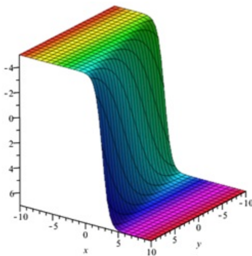
FIGURE 2. Kink wave u_3 at A = -\frac{1}{4} , B = 1 , C = 1 , D = 1 , \psi = 1 \lambda = 1 , a_0 = 1 , a_1 = 6 , z = 0.1 , and t = 0.2 .
