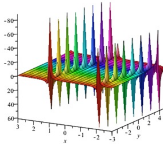
FIGURE 6. Degenerate wave solution u_{11} , for A = 0.1, B = 1, C = 1, D = 1, \psi = 2, \lambda = 2, a_0 = 1, a_1 = 6, z = 1, t = 2, c_1 = 1, \text{ and } c_2 = 2 .
