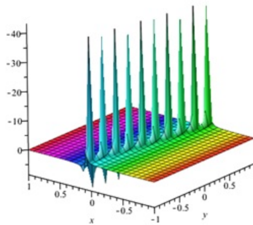
FIGURE 7. Soliton wave solution u_{12} for A = 0.2, B = 1, C = 1, D = 1, \psi = 2, \lambda = 3, a_0 = 1, a_1 = 6, z = 1, t = 2, c_1 = 1, \text{ and } c_2 = 2 .
