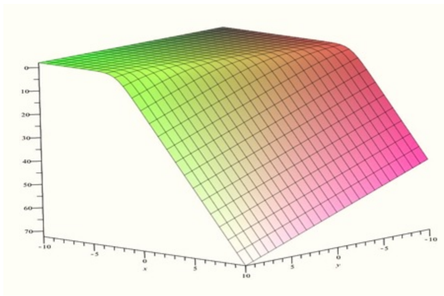
FIGURE 5. Typical breaking soliton wave solution u_8 at B = 1, C = 1, D = 1, \psi = 1, \lambda = 1, z = 0.1, t = 0.2, a_0 = 6, a_2 = -6 , and A = -0.25 .
