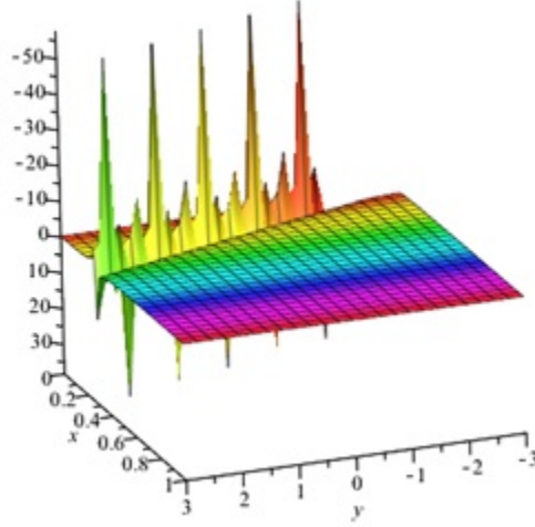
FIGURE 3. Soliton wave solution u_4 at B = 1 , C = 1 , D = 1 , \psi = 1 , \lambda = 1 , z = 0.1 , t = 0.2 , a_0 = 12 , a_2 = -6 , b_2 = -6 and A = -1/16 .
