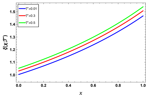
FIGURE 6. The graph shows the effect of changing \mathfrak{T} on the numerical solution for Equation (5.6) at M = 0.1, c = 1, q = 0.0001, \mathcal{X} \in [0, 1] .
