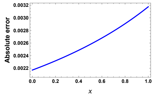
FIGURE 2. The absolute error between the analytical (4.7) and numerical (5.6) solutions at M = 0.1, c = 1, \mathfrak{T} = 0.01, q = 0.0001, \mathcal{X} \in [0, 1] .
