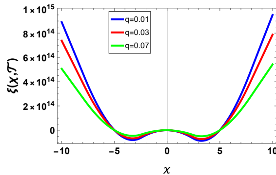
FIGURE 5. The graph shows the effect of q on the numerical solution for Equation (5.6) at M = 0.1, c = 1, \mathfrak{T} = 0.0001, \mathcal{X} \in [-10, 10] .
