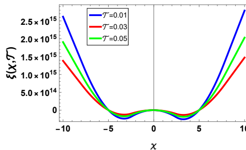
FIGURE 7. The graph shows the effect of changing \mathfrak{T} on the numerical solution for Equation (5.6) at M = 0.1, c = 1, q = 0.0001, \mathcal{X} \in [-10, 10] .
