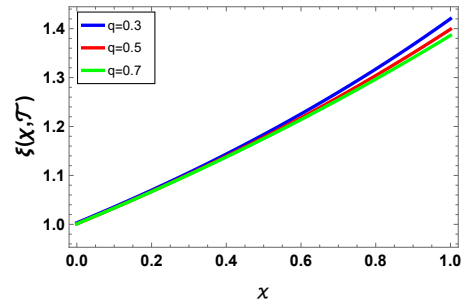
FIGURE 4. The graph shows the effect of q on the numerical solution for Equation (5.6) at M = 0.1, c = 1, \mathfrak{T} = 0.01, \mathcal{X} \in [0, 1] .
