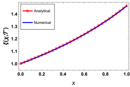
FIGURE 1. The graph shows the relation between the numerical and analytical solutions for (1.3) at M = 0.1, c = 1, \mathfrak{T} = 0.01, q = 0.0001, \mathcal{X} \in [0, 1] .
