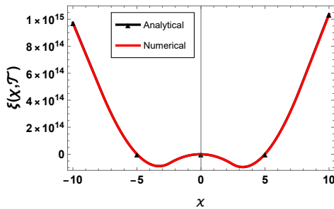
FIGURE 3. The graph shows the comparison between the numerical and analytical solutions for (1.3) at M = 0.1, c = 1, \mathfrak{T} = 0.0001, q = 0.0001, \mathcal{X} \in [-10, 10] .
