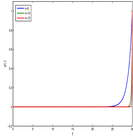
FIGURE 6. Solutions of the Troesch’s problem on time interval [0, 30] and different values of n .
