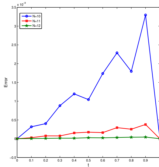
FIGURE 4. The error of the Troesch's problem with different number of CGL nodes, for n = 1 .
