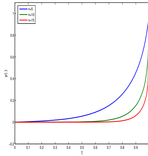
FIGURE 7. Solutions of the Troesch's problem on time interval [0, 1] and n = 5, 10, 15 .
