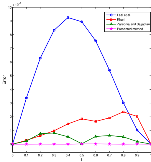
FIGURE 1. The error comparison of the CPS method with some other methods for n = 0.5 .
