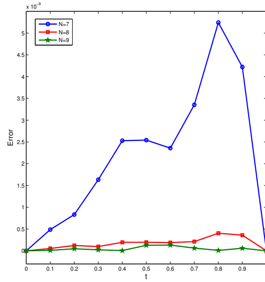
FIGURE 2. The error of the Troesch's problem with different number of CGL nodes, for n = 0.5 .
