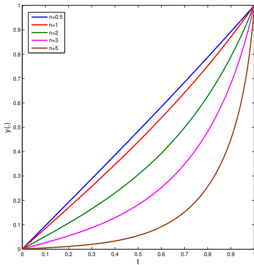
FIGURE 5. Solutions of the Troesch’s problem for different values of n .
