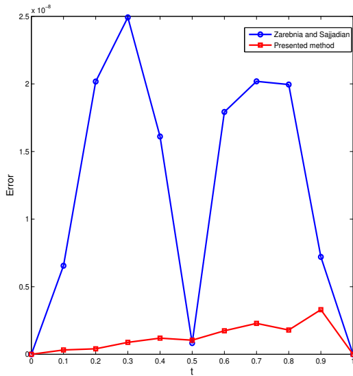
FIGURE 3. The error comparison of the CPS method with Zarebnia and Sajjadian method, for n = 1 and N = 10 .
