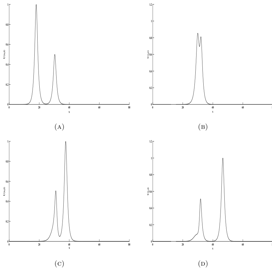
FIGURE 2. Graphs at A) t = 10 , B) t = 50 , C) t = 70 , D) t = 100 for p = 3 of two solitary wave interactions.
