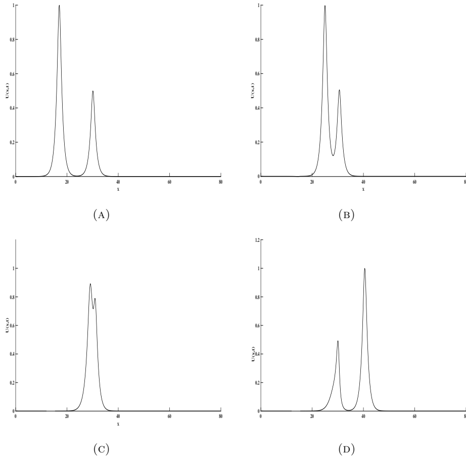
FIGURE 3. Graphs at A) t = 10 , B) t = 50 , C) t = 70 , D) t = 120 for p = 4 of two solitary wave interactions.
