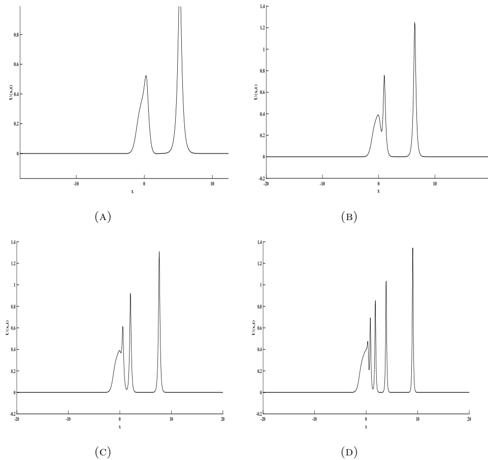
FIGURE 5. Maxwellian initial condition p = 4 , a) \mu = 0.1 , b) \mu = 0.05 , c) \mu = 0.025 , d) \mu = 0.01 at t = 12 .
