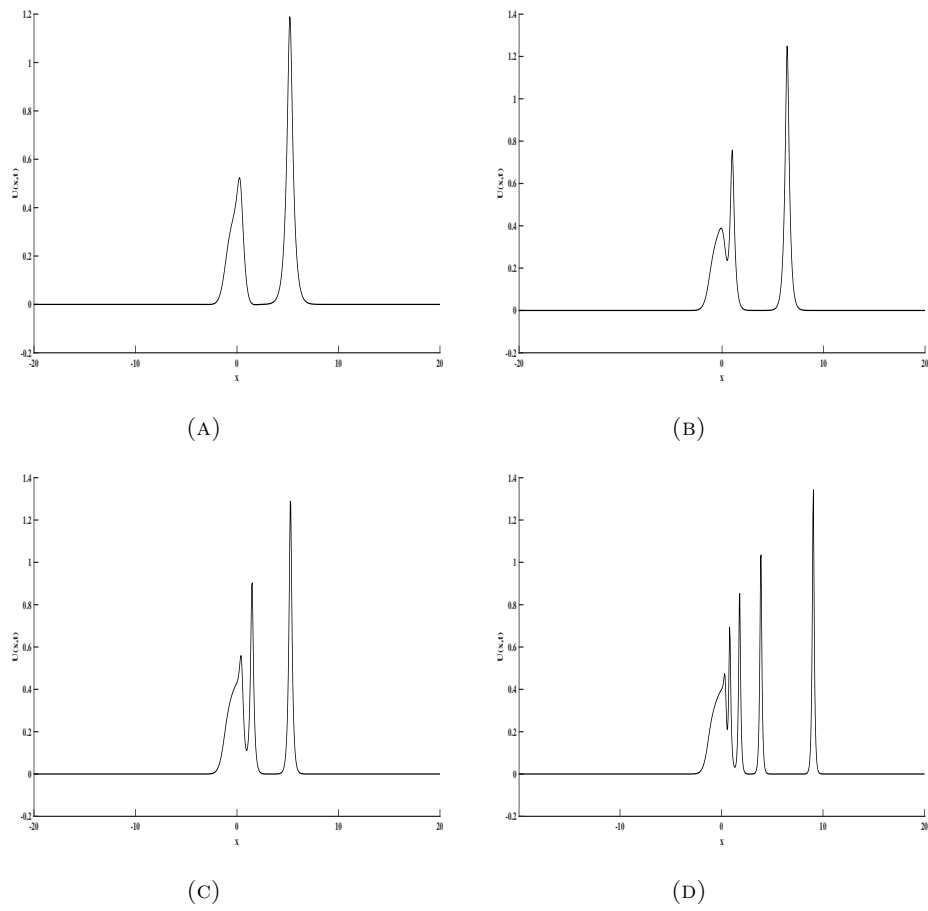
FIGURE 4. Maxwellian initial condition p = 3 , a) \mu = 0.1 , b) \mu = 0.05 , c) \mu = 0.025 , d) \mu = 0.01 at t = 12 .
