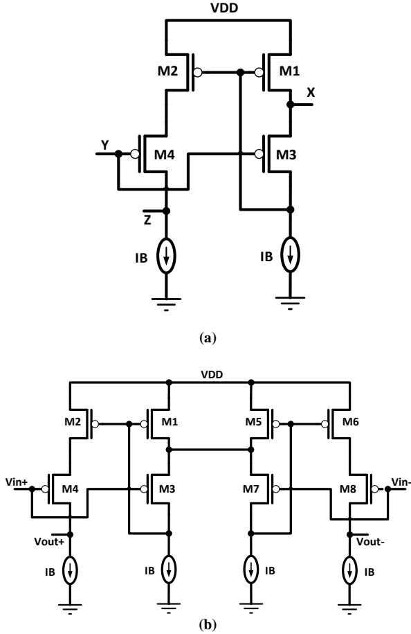
Fig. 2. (a) FVF-based CCII, (b) differential input stage based on FVF-based CCII
