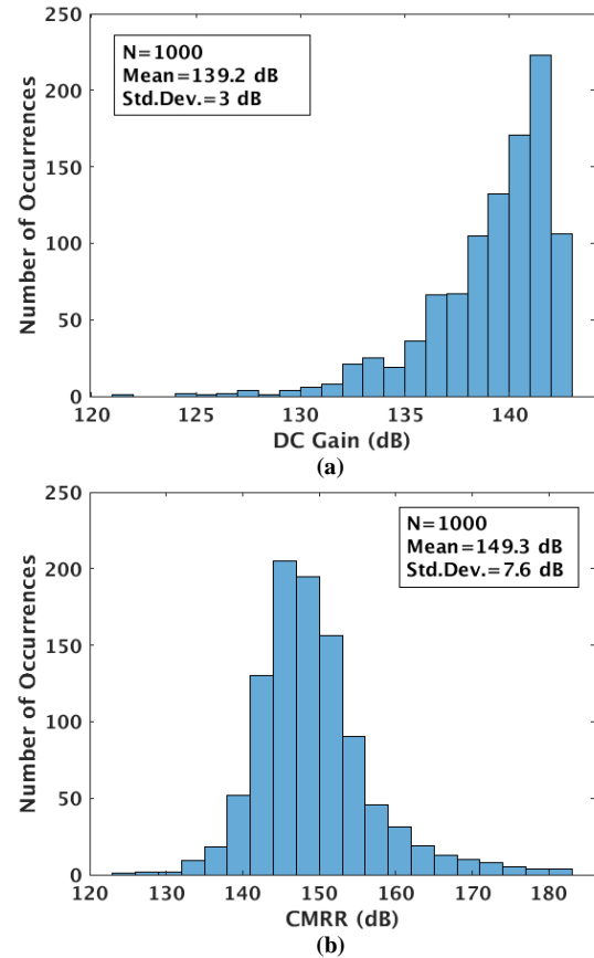
Fig. 10. The post-layout Monte Carlo simulation results for (a) DC voltage gain, (b) CMRR
