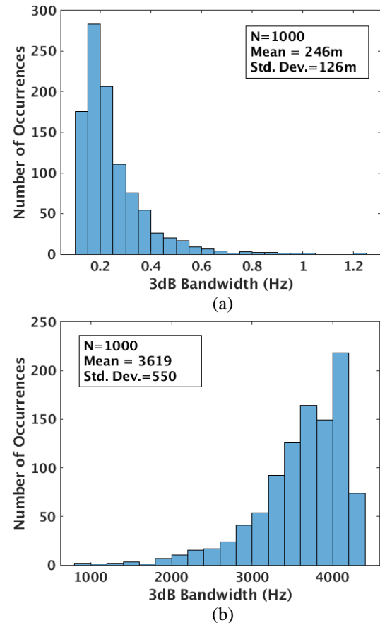
Fig. 11. The post-layout Monte Carlo simulation results for (a) Open loop bandwidth, (b) Closed loop bandwidth at 60 dB feedback gain
