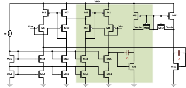
Fig. 3. Transistor level implementation of the proposed amplifier
