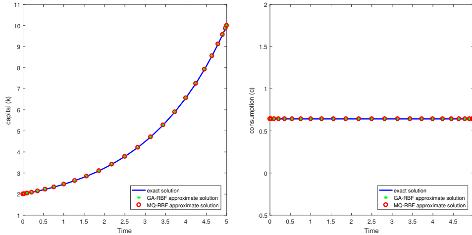
FIGURE 2. Solution to the optimal control Problem using GA-RBF and MQ RBF for N = 25 (a) capital (k), (b) consumption (c).
