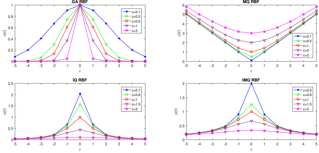
FIGURE 1. Figures of some well-known RBFs.
