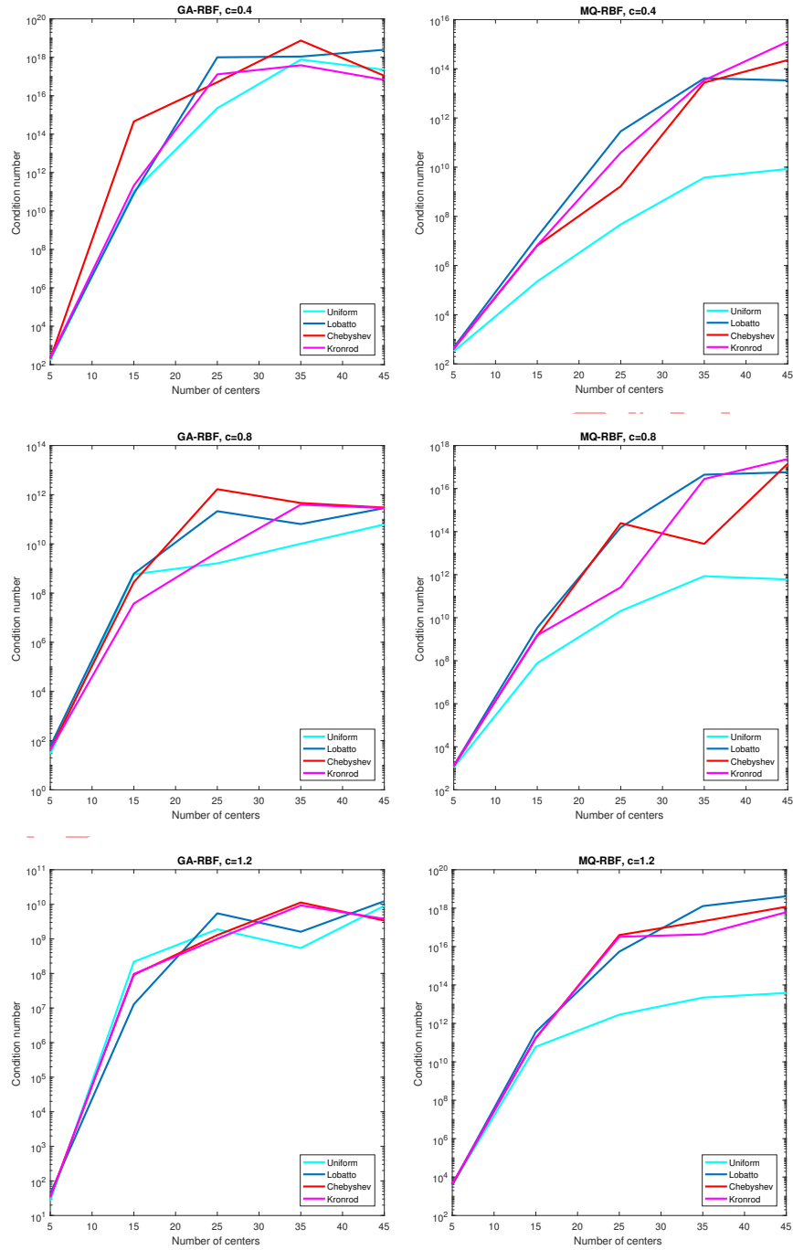
FIGURE 3. Behaviour of condition number when number of centers ( N ) increases for uniform, Gauss-Lobatto, Gauss-Chebyshev and Gauss-Kronrod centers points.
