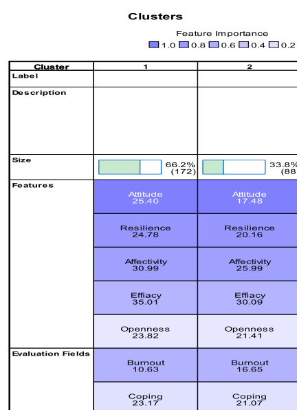
Figure 4. classification of clustering variables
