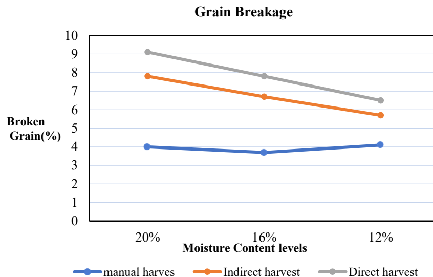
Fig 4. the effect of factor levels on fracture.
