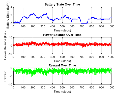
Fig. 4. Adaptive power balance control in hybrid microgrids using DRL and DT models.
