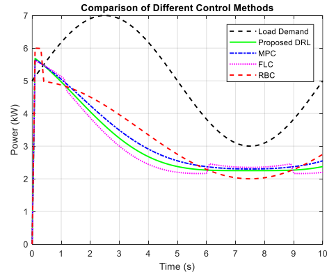
Fig. 10. Power balance comparison methods over time.
