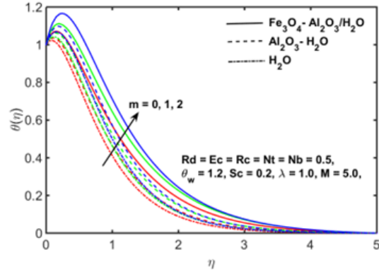
FIGURE 16. Effect of Hall current parameter ( m ) on \theta(\eta) .
