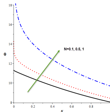
FIGURE 4. Effect of fin parameter on temperature distribution of Equation (3.31) at A = 1, B = 1, D = 10, t = 0.5 .
