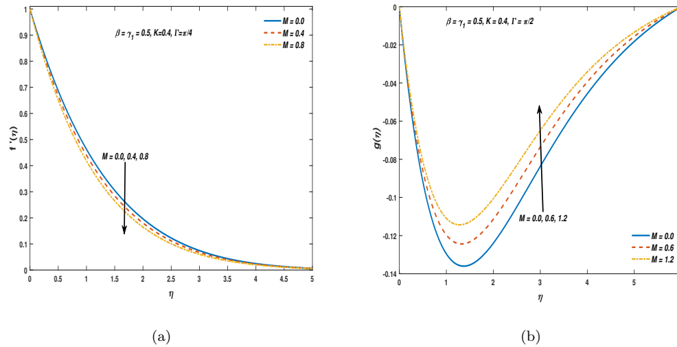
FIGURE 6. Velocity distributions against M .
