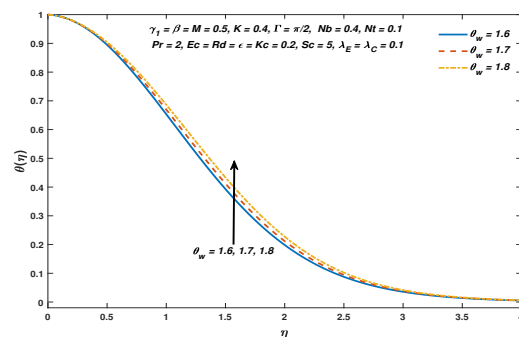
FIGURE 10. Temperature distribution against \theta_w .
