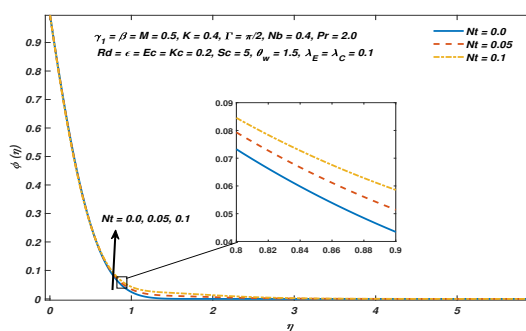
FIGURE 20. Concentration distribu- tion against Nt .
