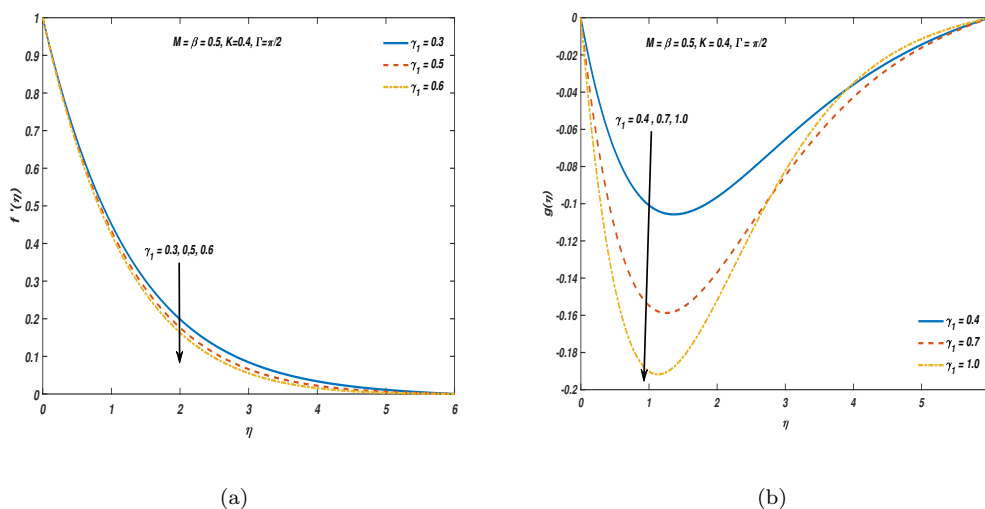
FIGURE 8. Velocity distributions against \gamma_1 .
