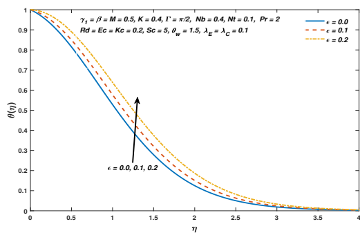
FIGURE 15. Temperature distribu- tion against \epsilon .
