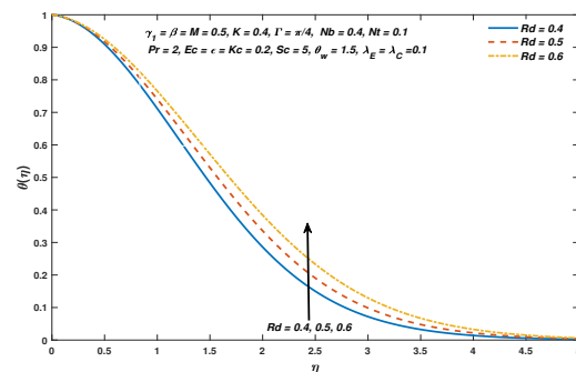
FIGURE 14. Temperature distribution against Rd .
