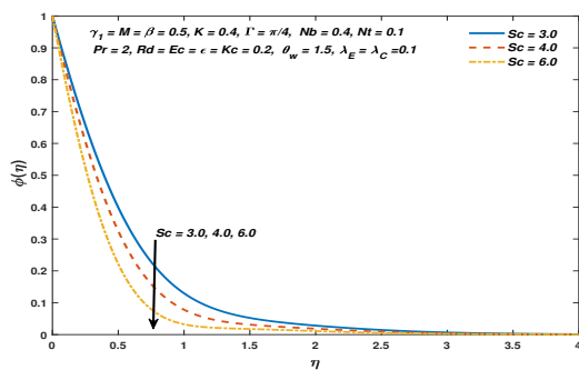
FIGURE 17. Concentration distribu- tion against Sc .
