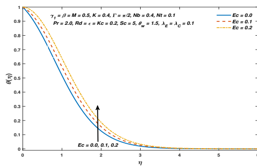
FIGURE 16. Temperature distribu- tion against Ec .
