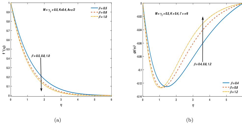
FIGURE 5. Velocity distributions against \beta .
