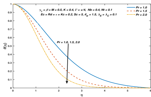
FIGURE 13. Temperature distribution against Pr .
