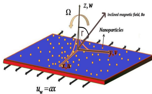
FIGURE 1. Geometry of physical model.
