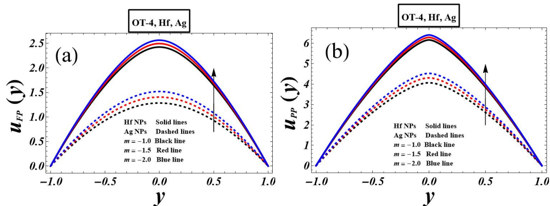
FIGURE 7. Impact of pressure gradient on fluid phase (a) and particulate phase (b) velocity.
