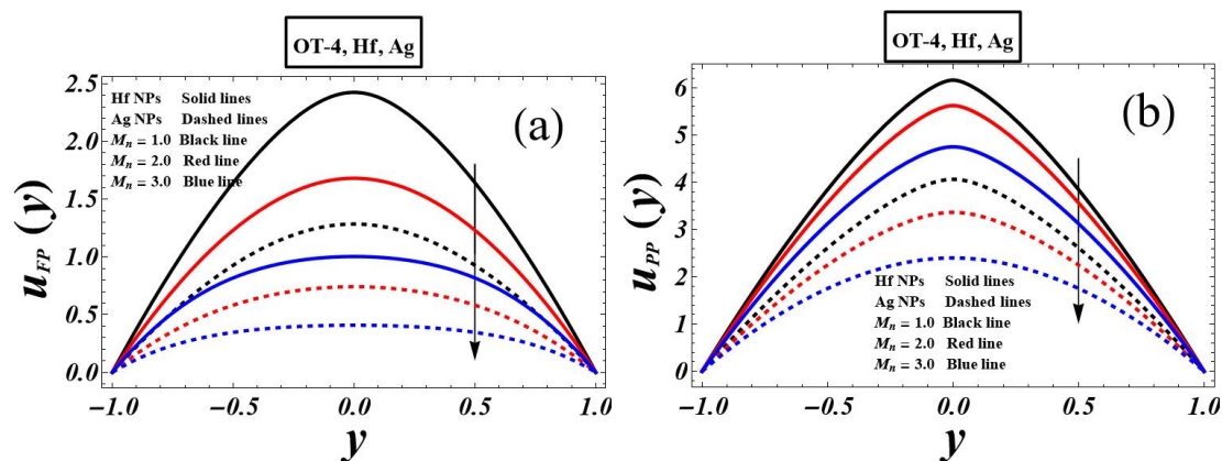
FIGURE 5. Impact of Hartman number on fluid phase (a) and particulate phase (b) velocity.
