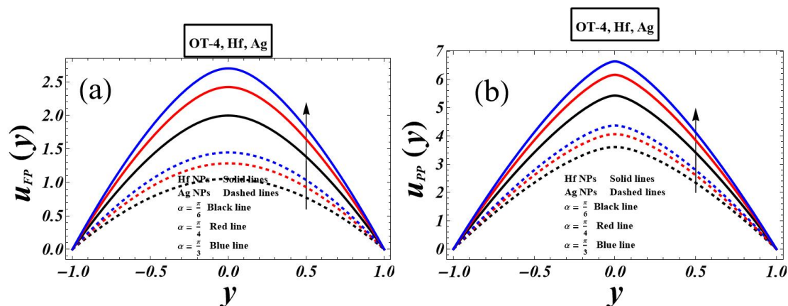
FIGURE 6. Impact of inclination angle on fluid phase (a) and particulate phase (b) velocity.
