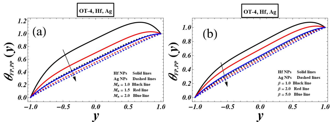
FIGURE 10. Impact of magnetic field parameter (a) and thermal radiation parameter (b) on thermal profile.
