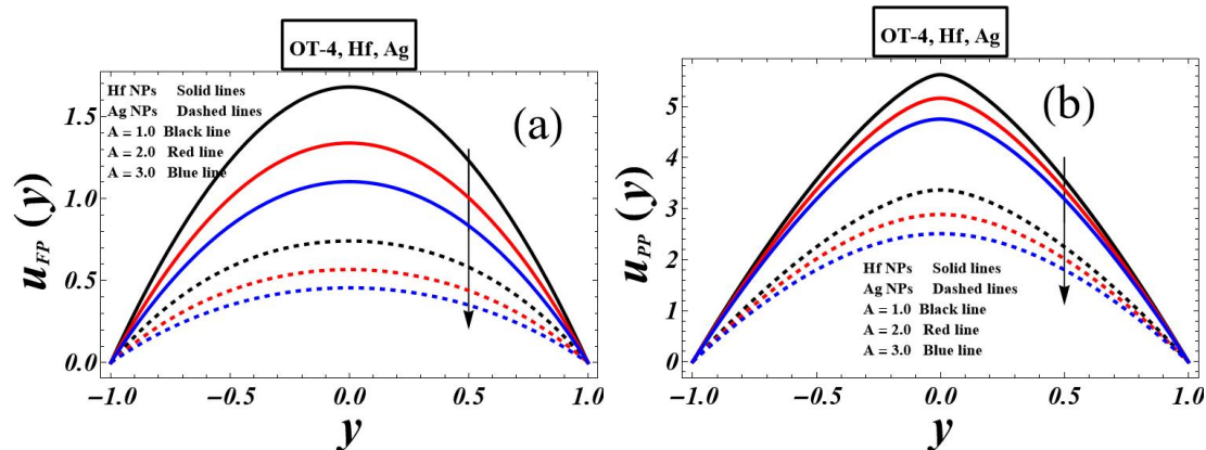
FIGURE 2. Impact of first Prandtl fluid parameter on fluid phase (a) and particulate phase (b) velocity.
