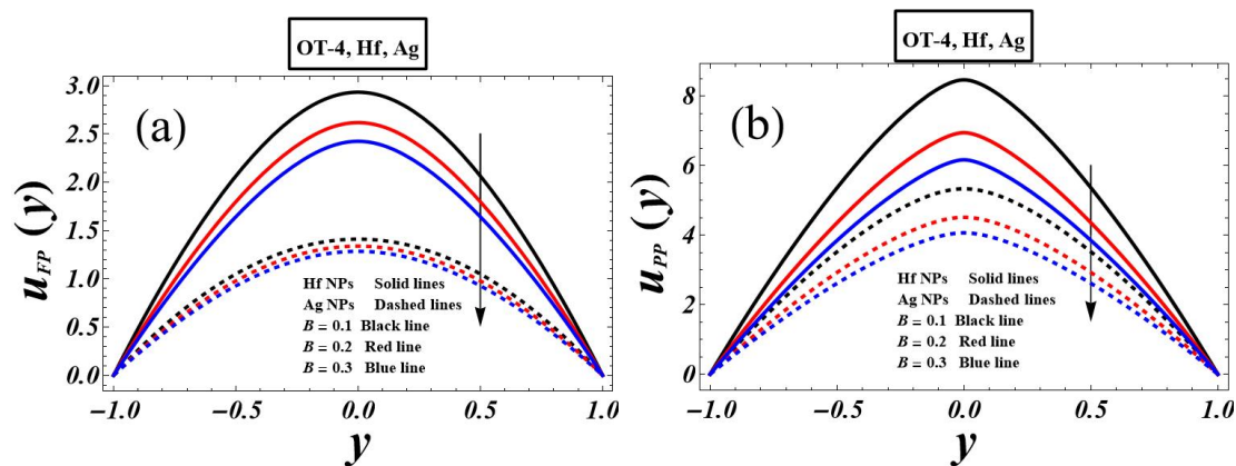
FIGURE 3. Impact of second Prandtl fluid parameter on fluid phase (a) and particulate phase (b) velocity.
