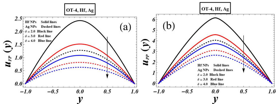
FIGURE 4. Impact of Froude number on fluid phase (a) and particulate phase (b) velocity.
