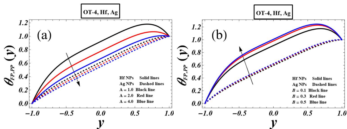
FIGURE 8. Impact of first Prandtl fluid parameter (a) and second Prandtl fluid parameter (b) on thermal profile.
