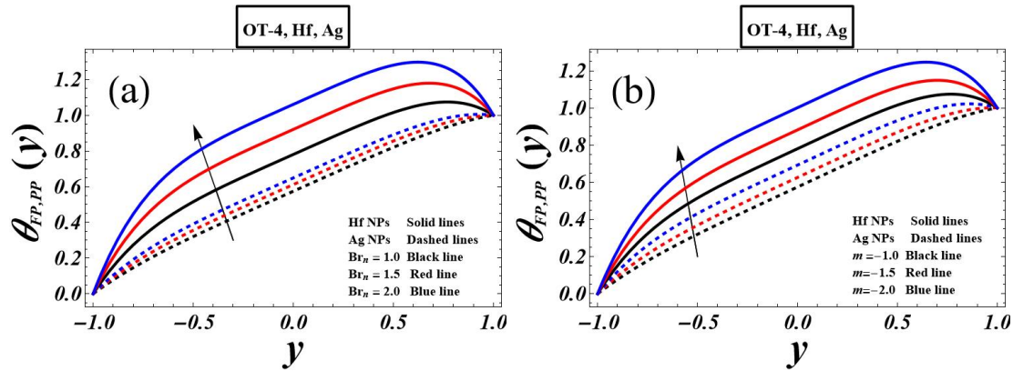
FIGURE 11. Impact of Brinkman number (a) and pressure gradient parameter (b) on thermal profile.
