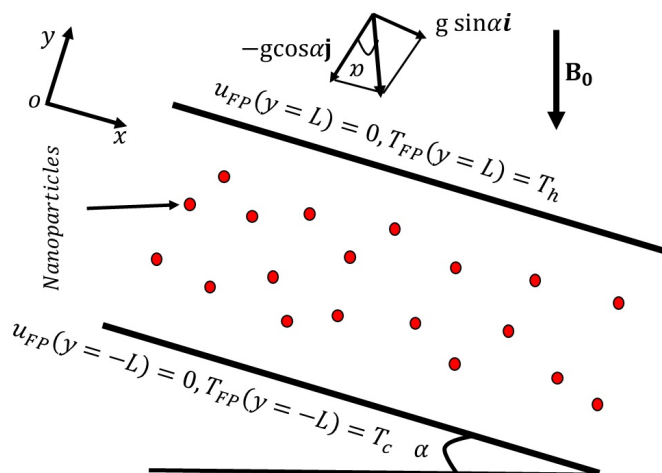
FIGURE 1. Flow configuration.
