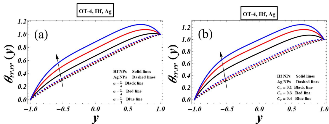
FIGURE 9. Impact of angle of inclination (a) and density number (b) on thermal profile.
