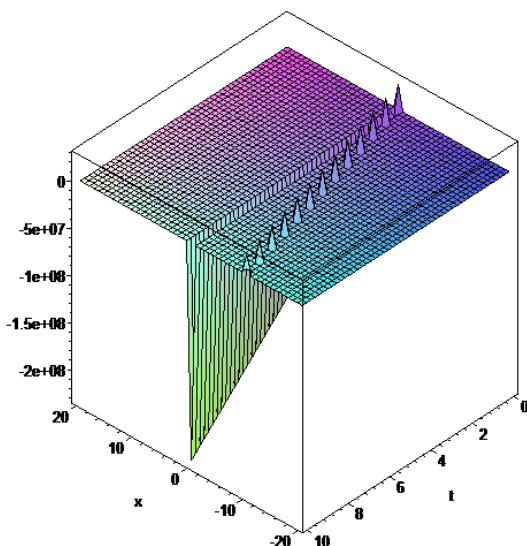
FIGURE 1. The solution of Case 3 considering the parameters of Set 1 for c_2 = 1 , c_1 = 1 , \lambda_2 = -3 , \lambda_1 = -1 .
