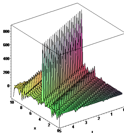
FIGURE 2. The solution of Case 4 for a_0 = 1 , c_1 = 1 , c_2 = -1 , \lambda = 1 .
