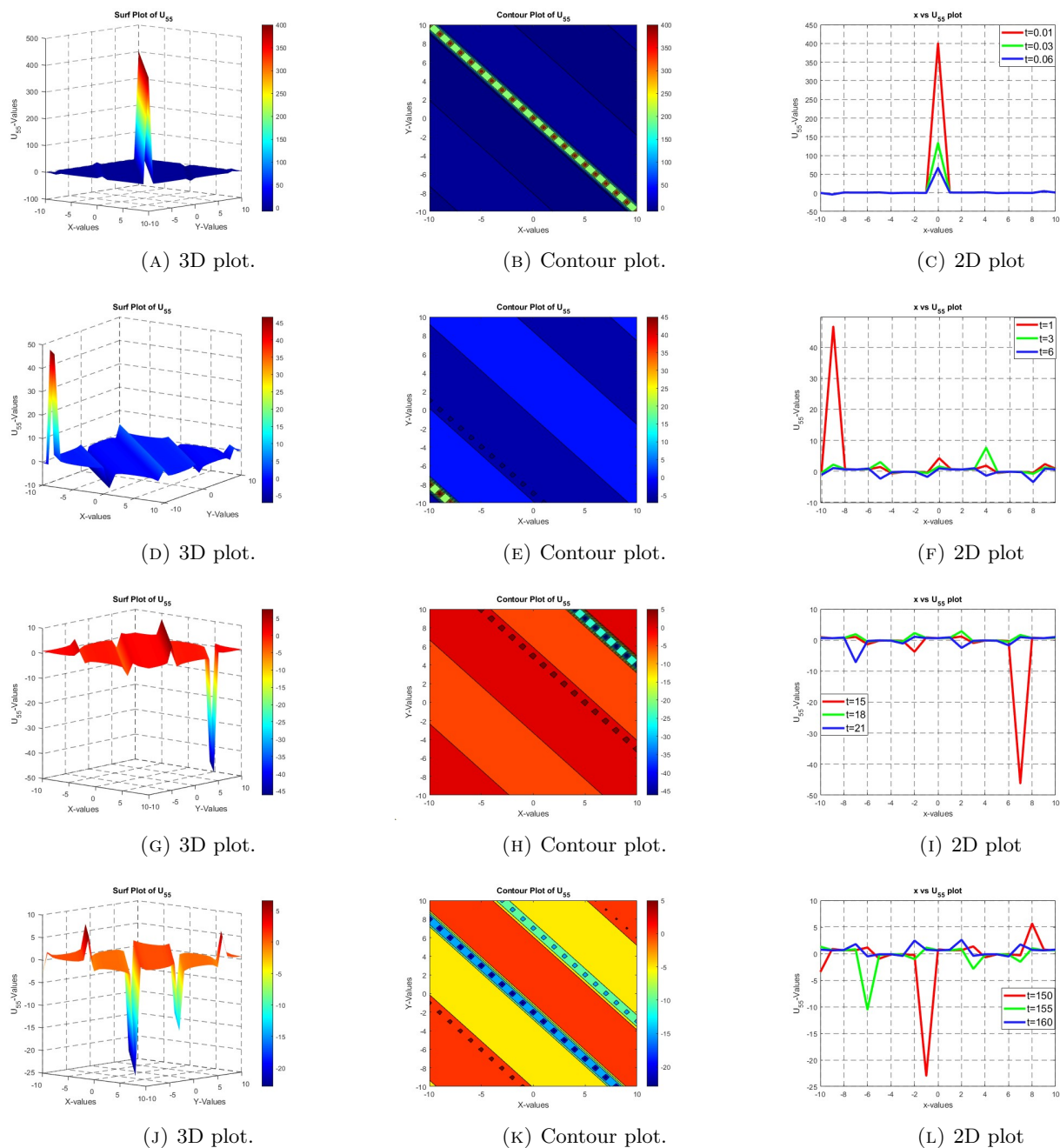
FIGURE 6. Shapes for Equation (3.33).
