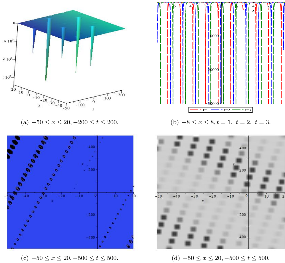
FIGURE 2. Wave profile of \phi_7 for p = 2 , q = 2 , r = 0 , and k = 1 .
