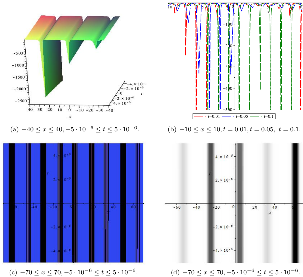
FIGURE 9. Wave profile of \phi_{61} for p = -2 , q = -2 , r = 0 , and k = 1 .
