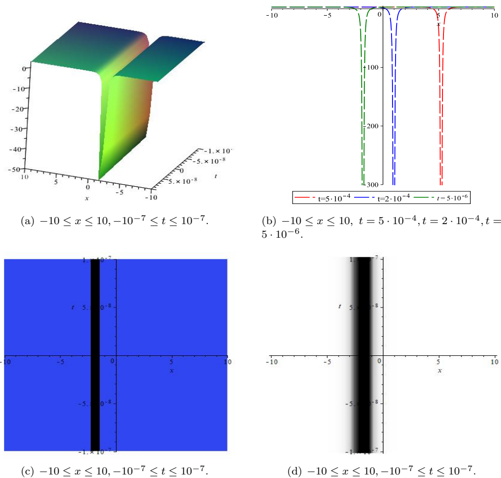
FIGURE 4. Wave profile of \phi_{13} for p = 1, q = 1, r = 3, \eta_0 = 1 , and k = 1 .
