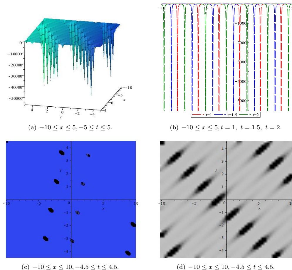
FIGURE 5. Wave profile of \phi_{15} for p = 1 , q = 2 , r = 1 , \eta_0 = 1 , and k = 1 .
