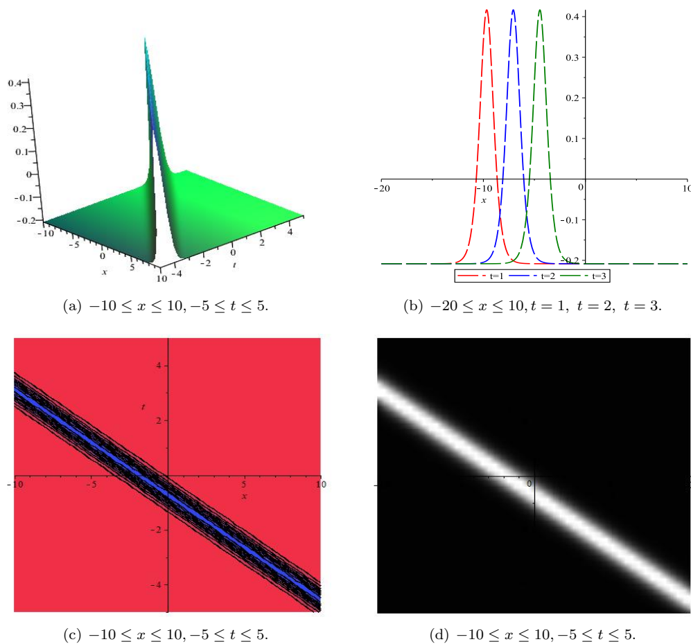
FIGURE 8. Wave profile of \phi_{54} for p = 1 , q = 1 , r = 3 , and k = 1 .
