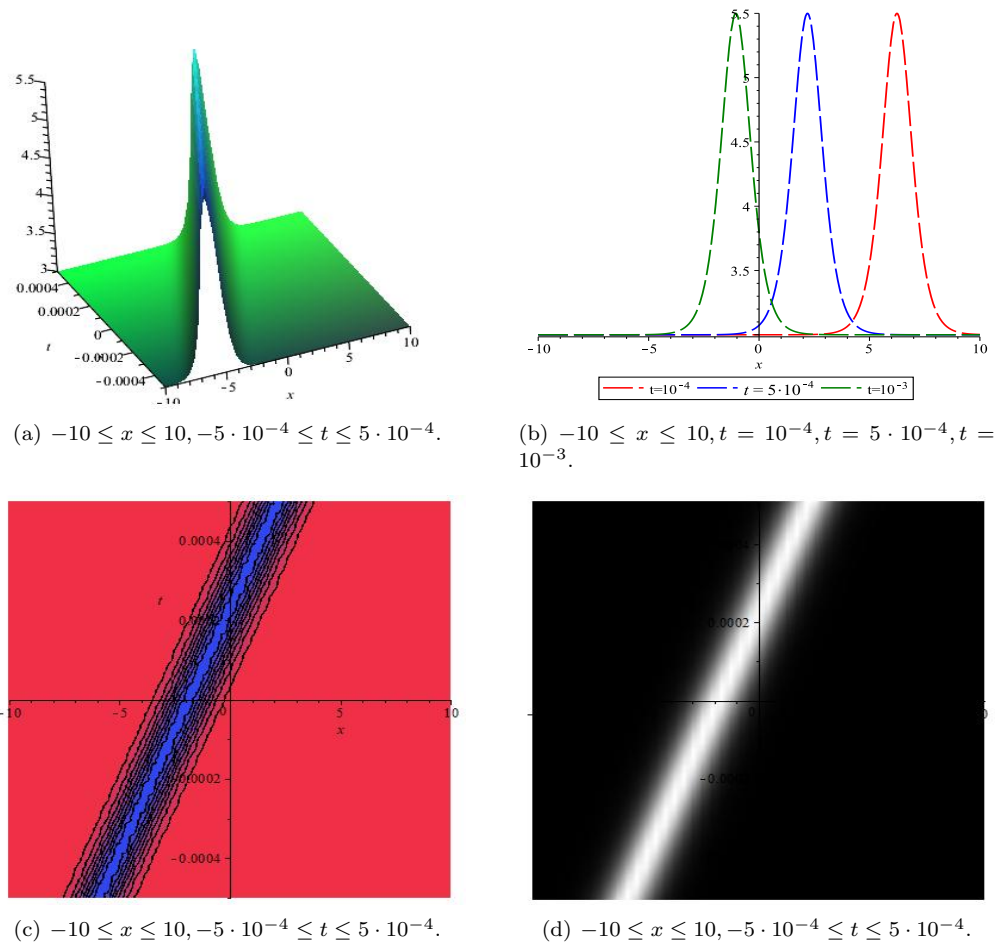
FIGURE 6. Wave profile of \phi_{43} for p = 1, q = 1, r = 3, \eta_0 = 1 , and k = 1 .
