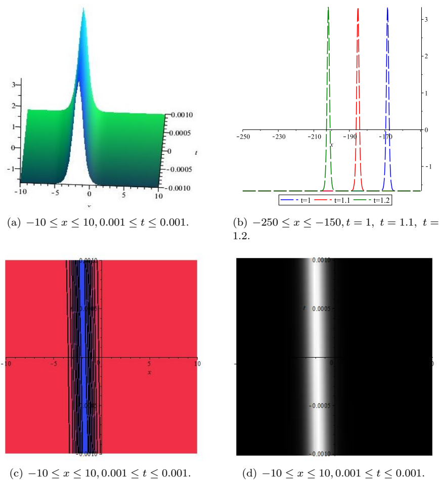
FIGURE 1. Wave profile of \phi_1 for p = 1 , q = 1 , r = 3 , and k = 1 .
