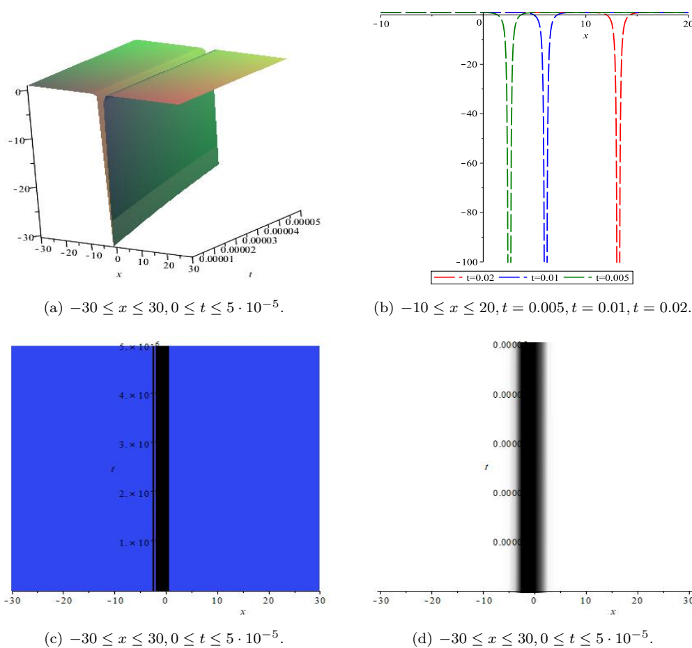
FIGURE 7. Wave profile of \phi_{47} for p = 1 , q = 2 , r = 1 , \eta_0 = 1 , and k = 1 .
