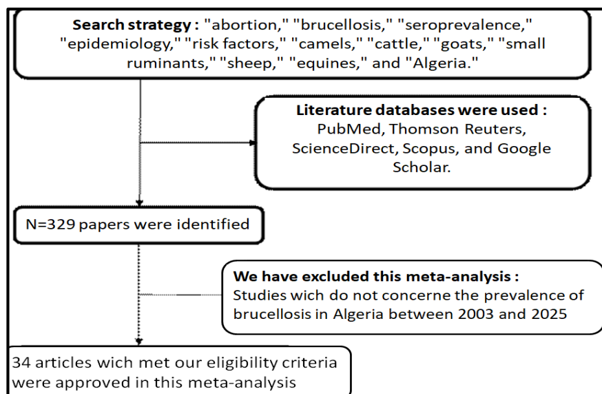
Fig. 1. Flowchart showing study inclusion and exclusion criteria
