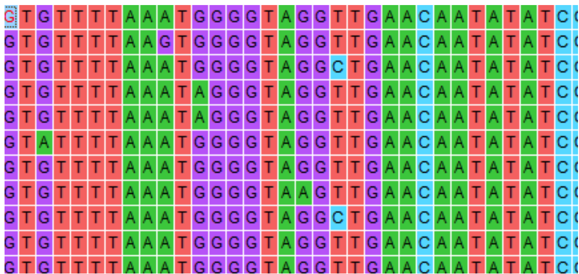
Figure 1. Multiple sequence alignment of mitochondrial COI gene fragments from Coccinella septempunctata populations using MEGA software.
