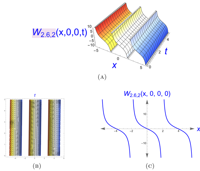
FIGURE 2. The singular periodic wave solution for Eq. (3.25).
