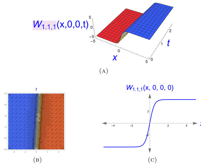
FIGURE 1. The dark soliton solution for Eq. (3.5).
