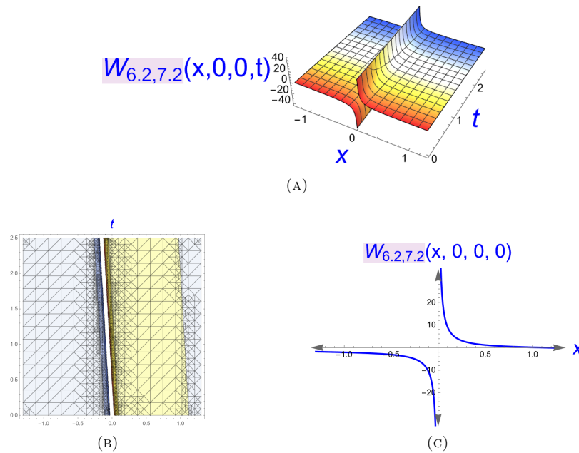
FIGURE 4. The combo dark-singular solution for Eq. (3.66).
