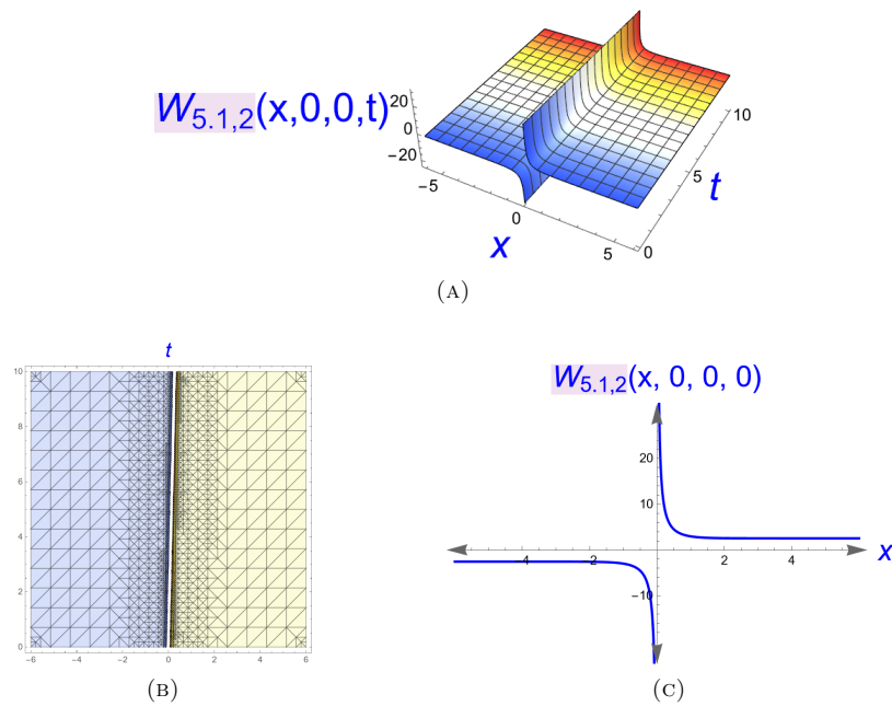
FIGURE 3. The singular soliton solution for Eq. (3.35).
