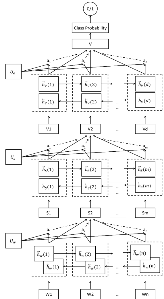
Fig. 2. Hierarchical Attention Network Plus (HAN+) Architecture.
