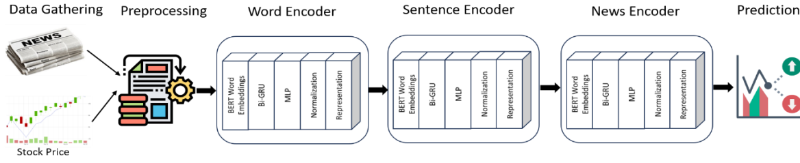
Fig. 3. The step-by-step flowchart of HAN+BERT.
