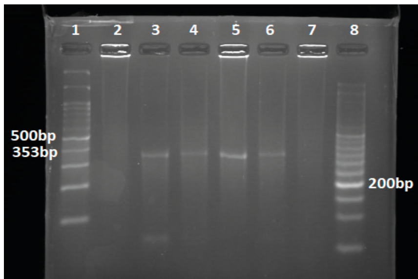
Fig. 2. Agarose gel image of the amplified fragment of Pasteurella spp. The 16srRNA gene (353 nucleotides) was amplified by PCR. The first lane is a 100-bp ladder, and the eighth lane is 50-bp ladder (both from Smobio Technology Inc., Taiwan). Lanes 3 to 6 are positive for Pasteurella spp., lane 2 is a negative control, and lane 7 is a negative examples.
