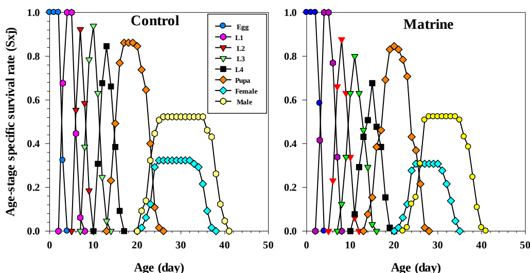
Figure. 1. Age-stage specific survival rate ( S_{xj} ) of Tuta absoluta exposed to sublethal concentration ( LC_{25} ) of Matrine and control treatment.
